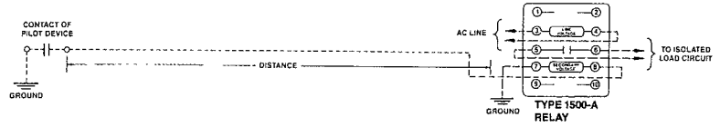
Single conductor remote control using ground return.
